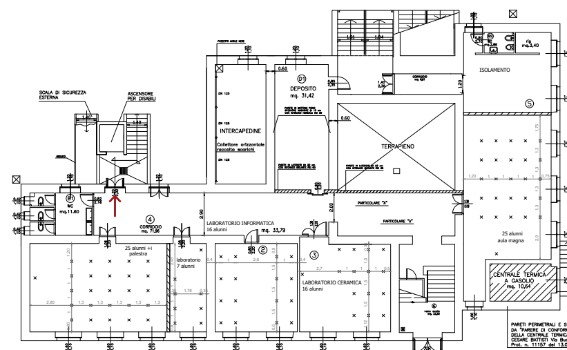
PIANO INTERRATO
